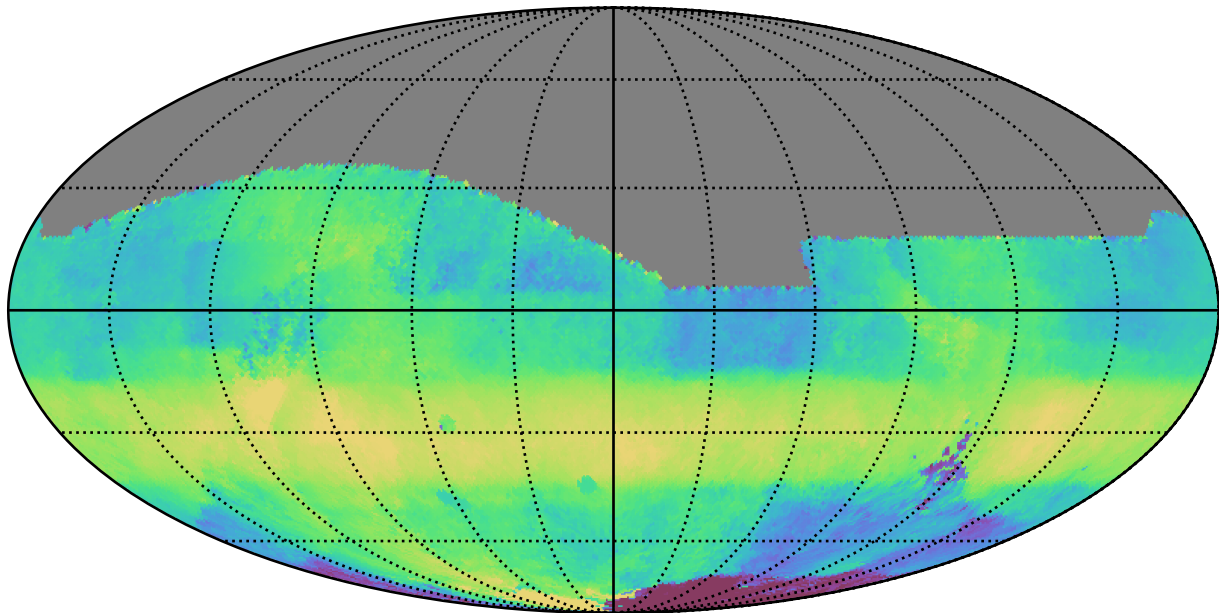
ddf_acor_sf10_lsf20_lsr10_v3.4_10yrs All sky r band: Median HA
