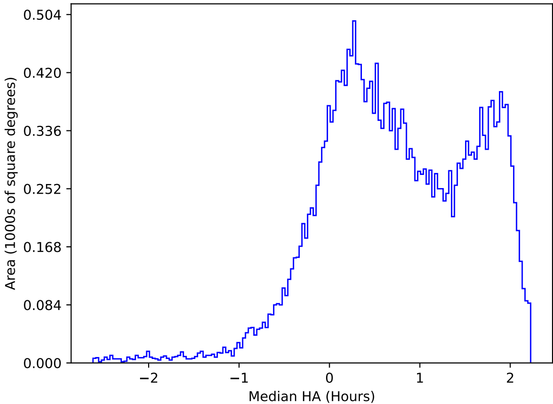
ddf_acor_sf10_lsf20_lsr10_v3.4_10yrs All sky r band: Median HA
