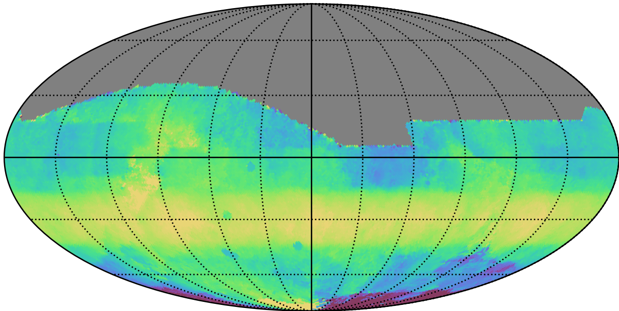
ddf_acor_sf10_lsf20_lsr10_v3.4_10yrs All sky i band: Median HA
