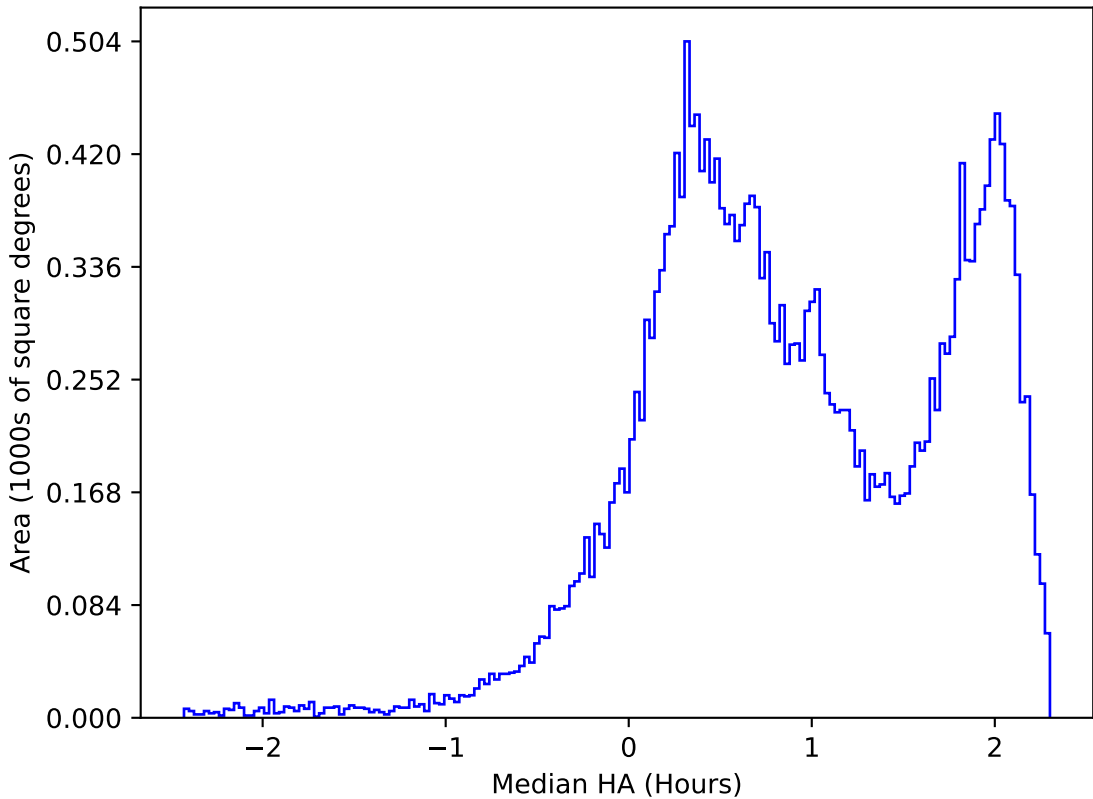
ddf_acor_sf10_lsf20_lsr10_v3.4_10yrs All sky i band: Median HA
