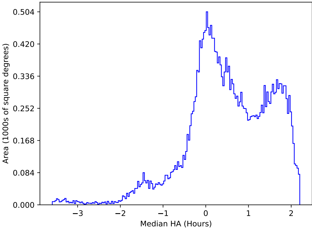
ddf_acor_sf10_lsf20_lsr10_v3.4_10yrs All sky g band: Median HA
