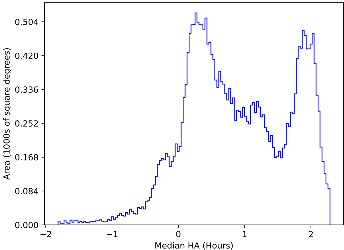
ddf_acor_sf10_lsf20_lsr10_v3.4_10yrs All sky all bands: Median HA
