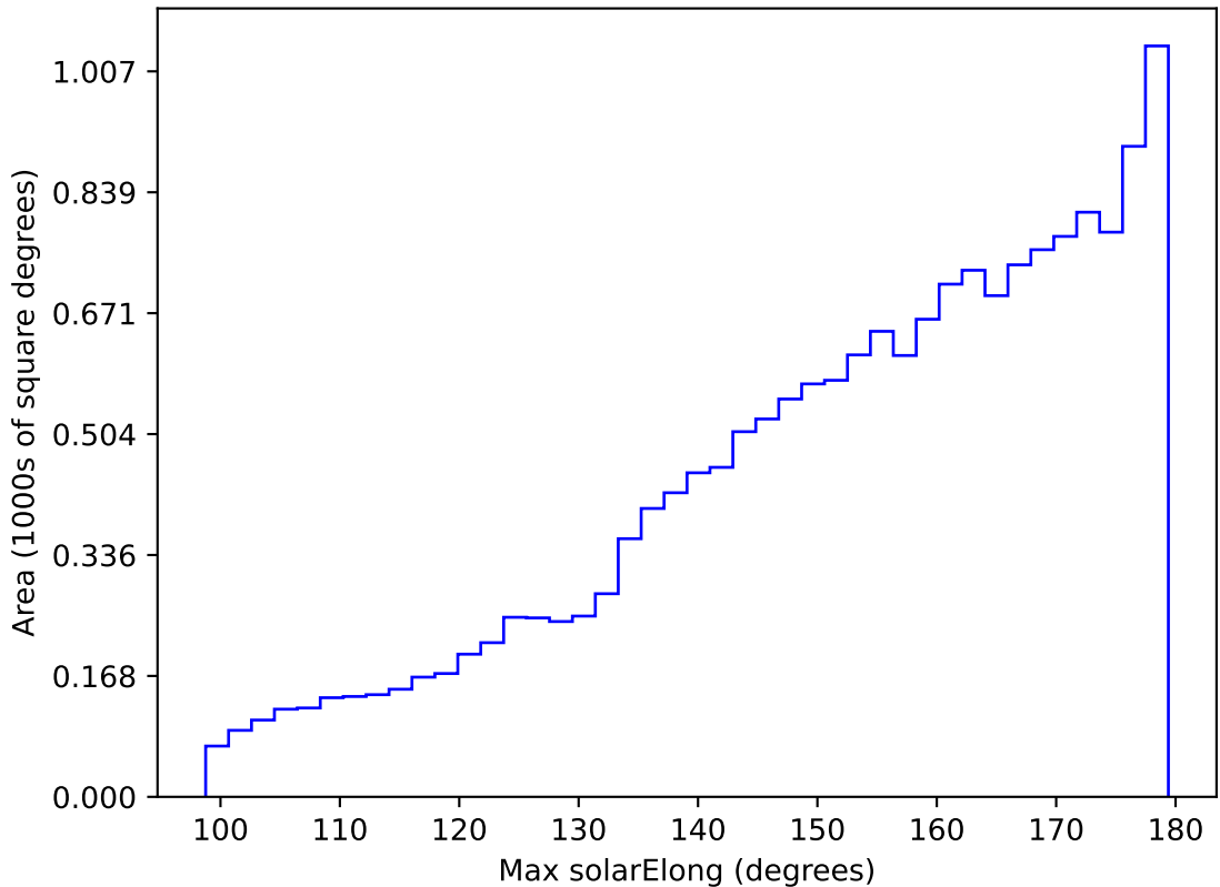
ddf_acor_sf10_lsf20_lsr10_v3.4_10yrs WFD z band: Max solarElong
