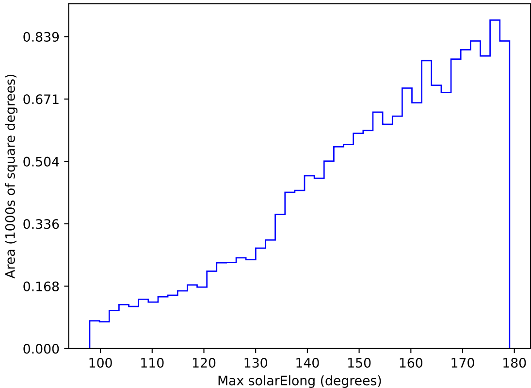
ddf_acor_sf10_lsf20_lsr10_v3.4_10yrs WFD u band: Max solarElong
