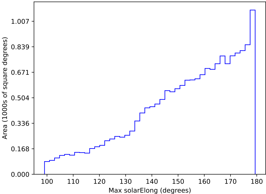
ddf_acor_sf10_lsf20_lsr10_v3.4_10yrs WFD r band: Max solarElong
