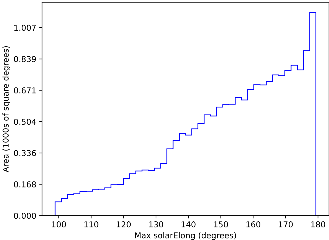
ddf_acor_sf10_lsf20_lsr10_v3.4_10yrs WFD i band: Max solarElong
