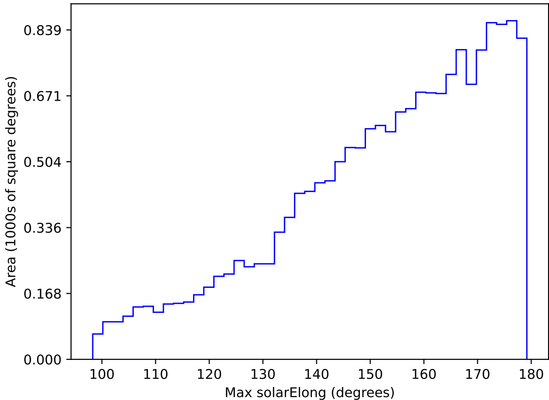
ddf_acor_sf10_lsf20_lsr10_v3.4_10yrs WFD g band: Max solarElong
