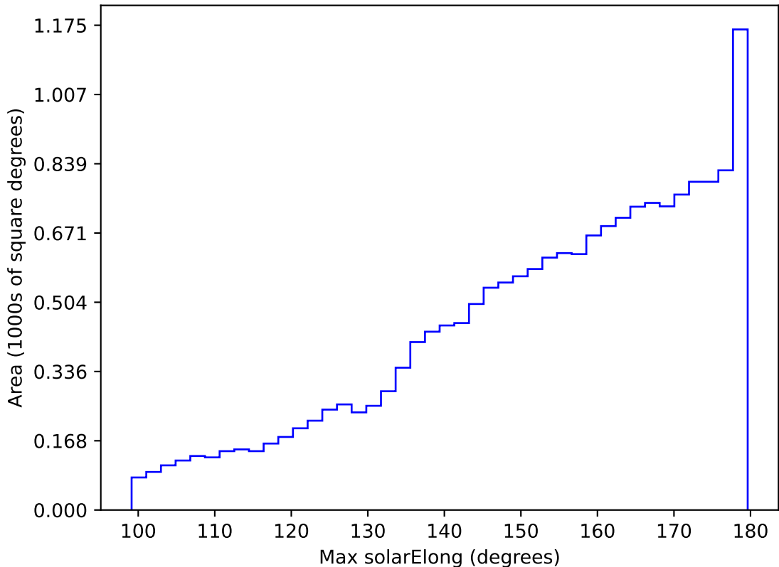
ddf_acor_sf10_lsf20_lsr10_v3.4_10yrs WFD all bands: Max solarElong
