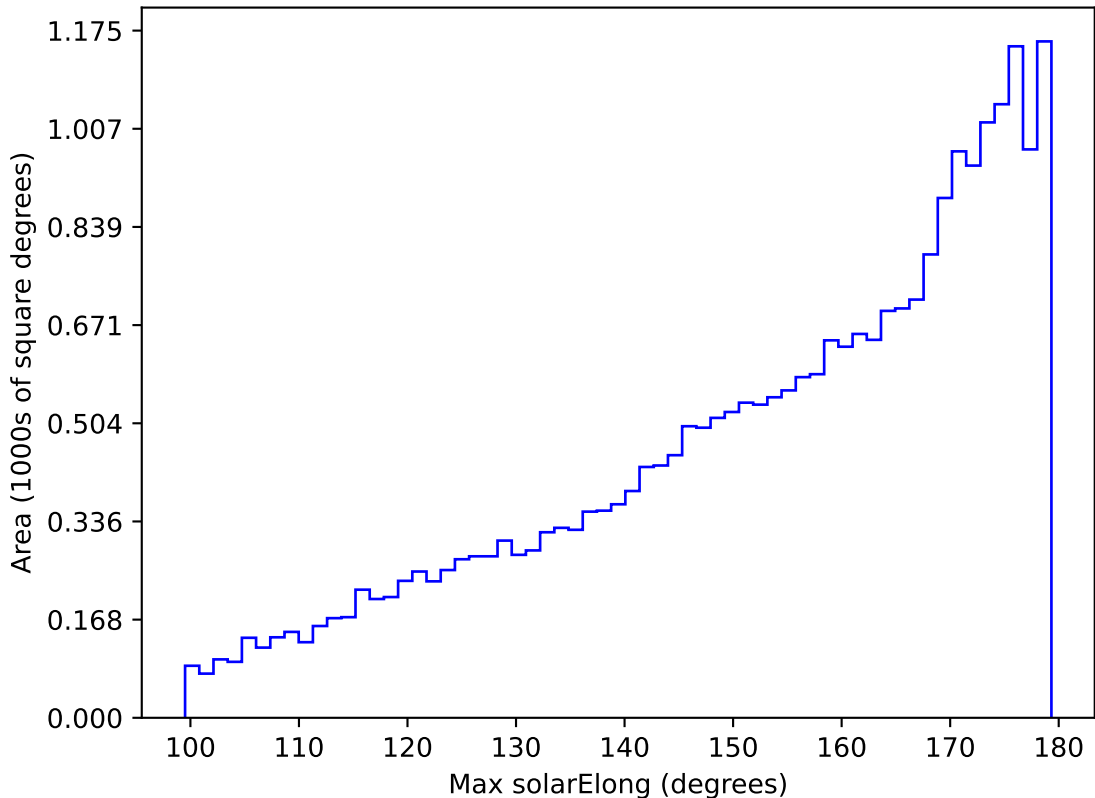
ddf_acor_sf10_lsf20_lsr10_v3.4_10yrs All sky z band: Max solarElong
