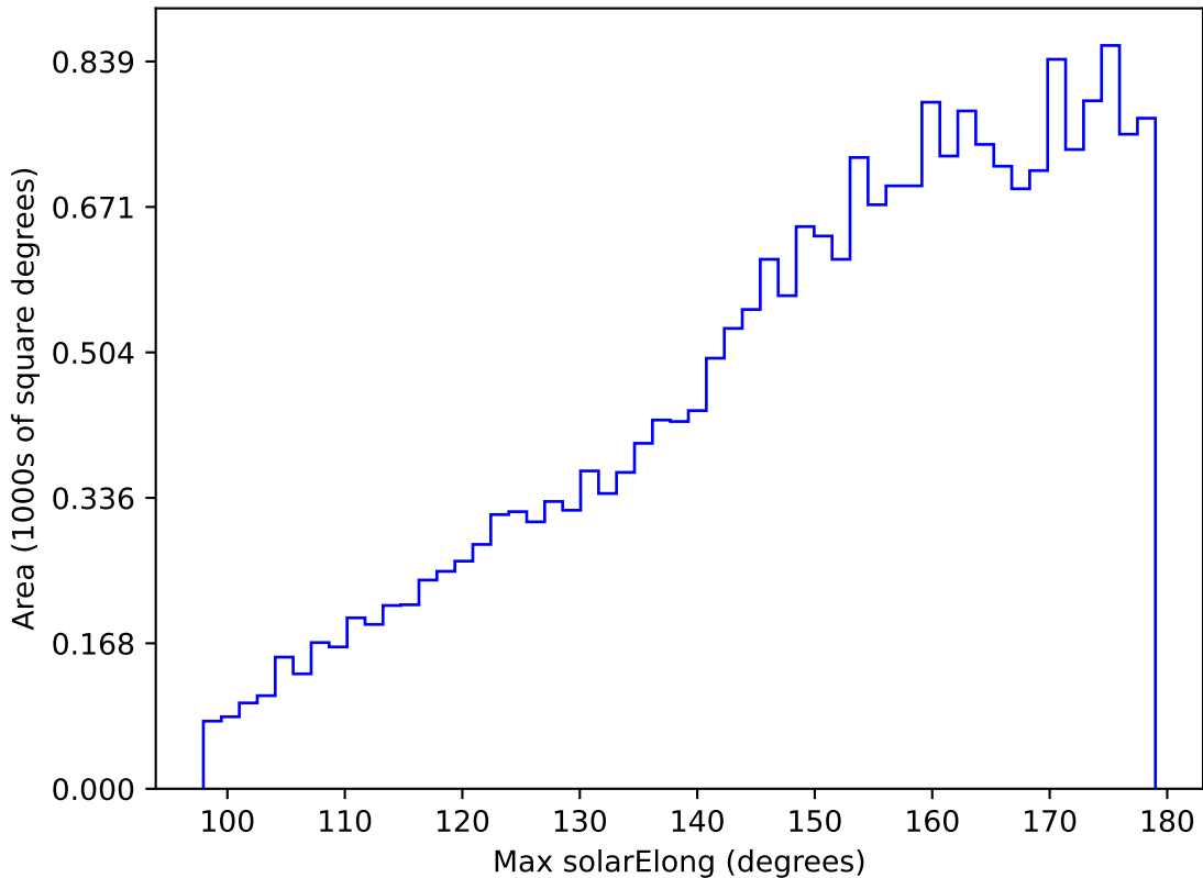
ddf_acor_sf10_lsf20_lsr10_v3.4_10yrs All sky u band: Max solarElong
