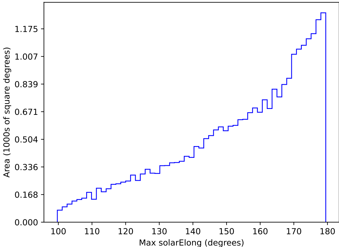
ddf_acor_sf10_lsf20_lsr10_v3.4_10yrs All sky r band: Max solarElong
