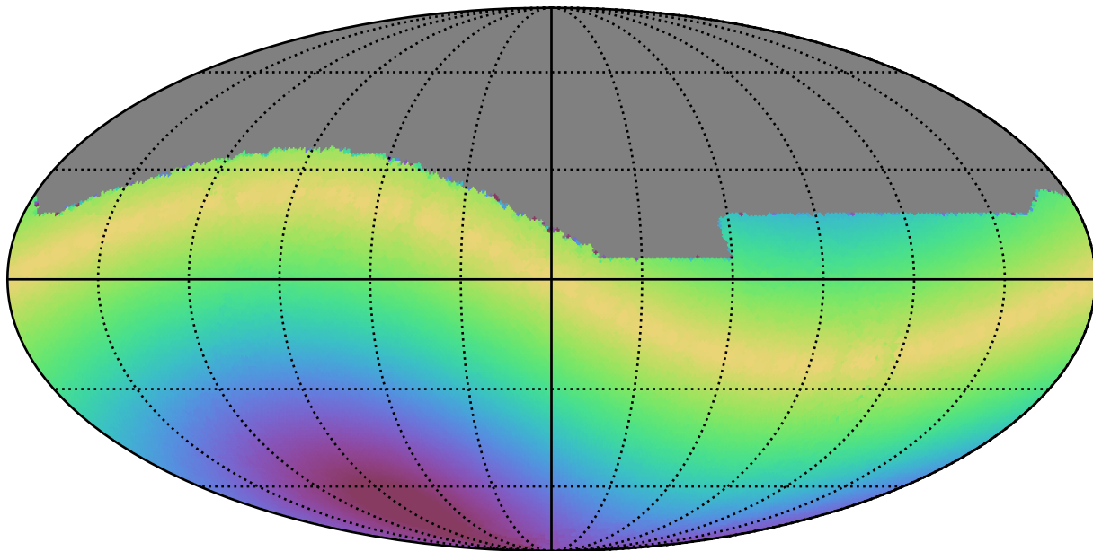
ddf_acor_sf10_lsf20_lsr10_v3.4_10yrs All sky i band: Max solarElong
