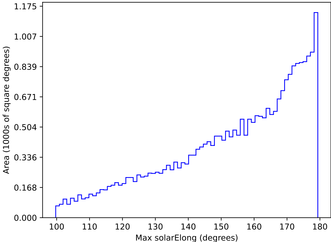
ddf_acor_sf10_lsf20_lsr10_v3.4_10yrs All sky i band: Max solarElong
