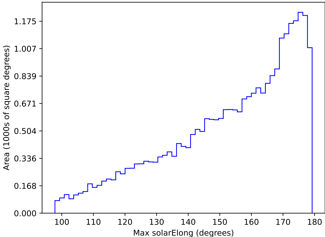
ddf_acor_sf10_lsf20_lsr10_v3.4_10yrs All sky g band: Max solarElong
