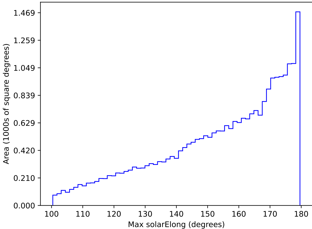
ddf_acor_sf10_lsf20_lsr10_v3.4_10yrs All sky all bands: Max solarElong
