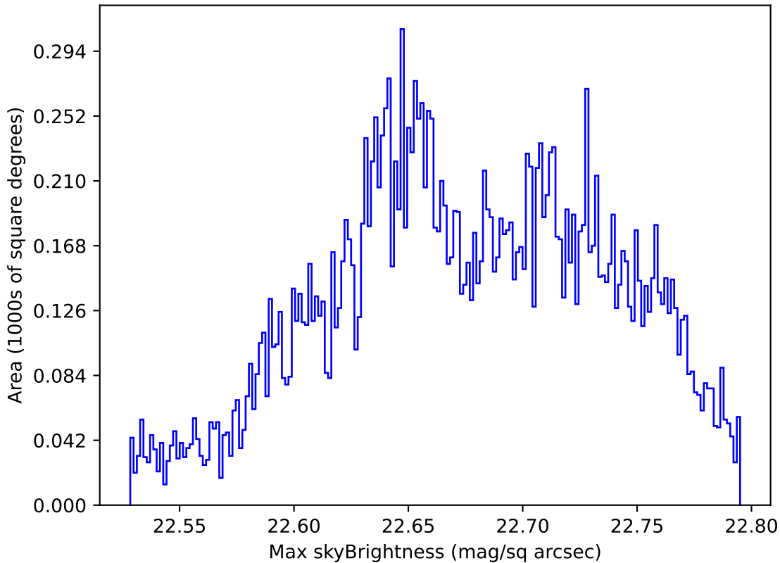
ddf_acor_sf10_lsf20_lsr10_v3.4_10yrs Yr 1 u band: Max skyBrightness
