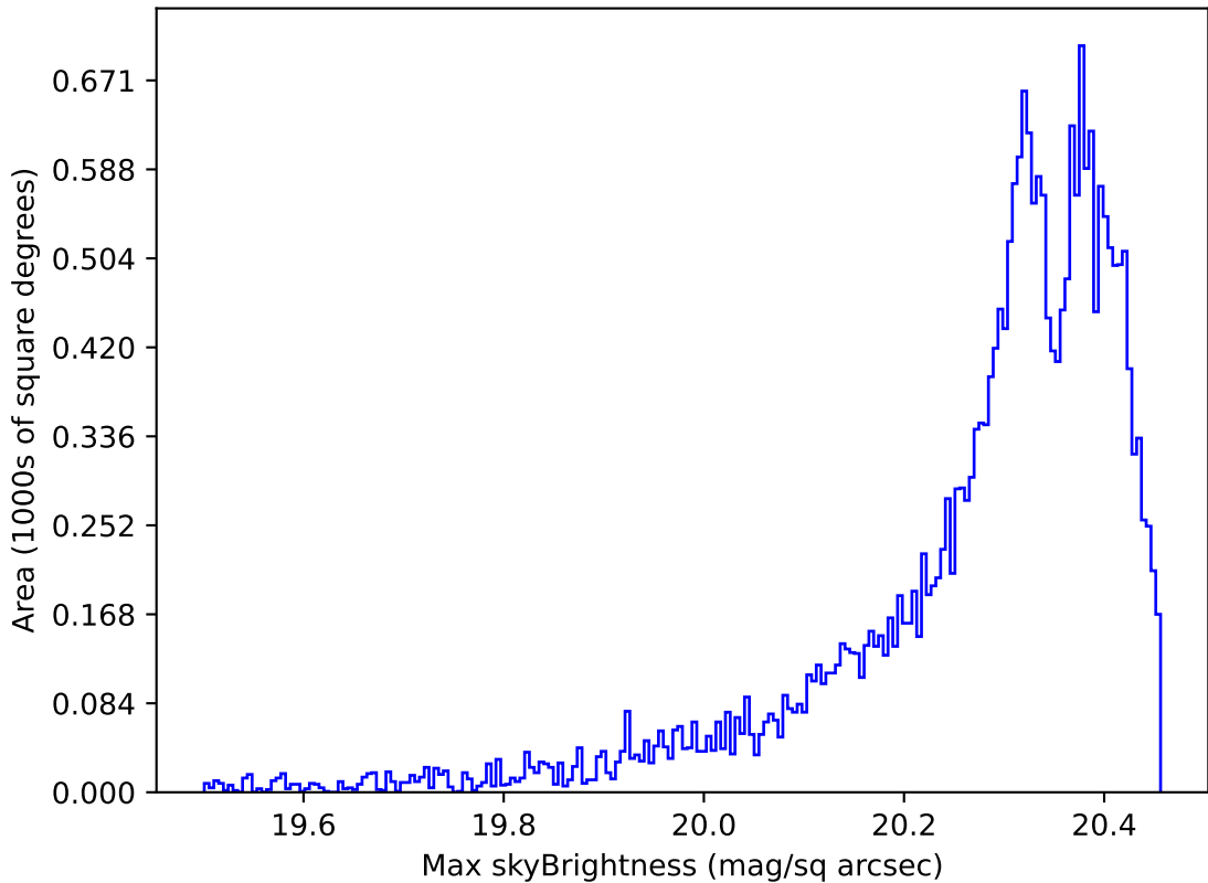
ddf_acor_sf10_lsf20_lsr10_v3.4_10yrs Yr 1 i band: Max skyBrightness
