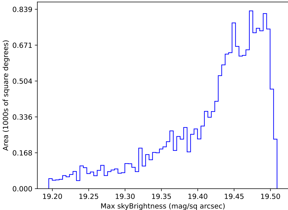
ddf_acor_sf10_lsf20_lsr10_v3.4_10yrs WFD z band: Max skyBrightness
