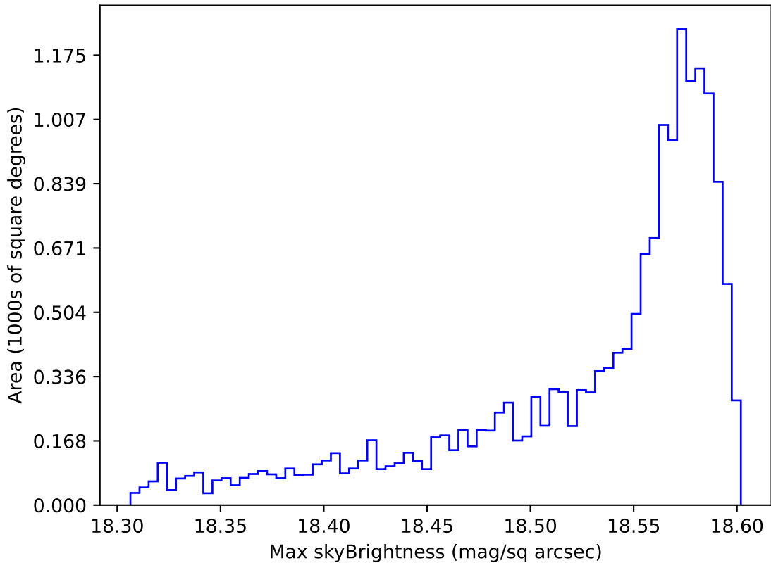
ddf_acor_sf10_lsf20_lsr10_v3.4_10yrs WFD y band: Max skyBrightness
