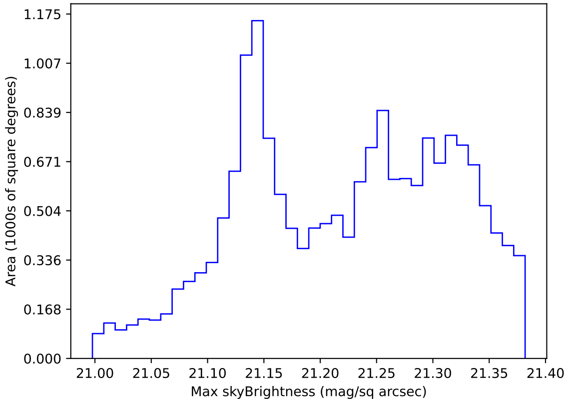
ddf_acor_sf10_lsf20_lsr10_v3.4_10yrs WFD r band: Max skyBrightness
