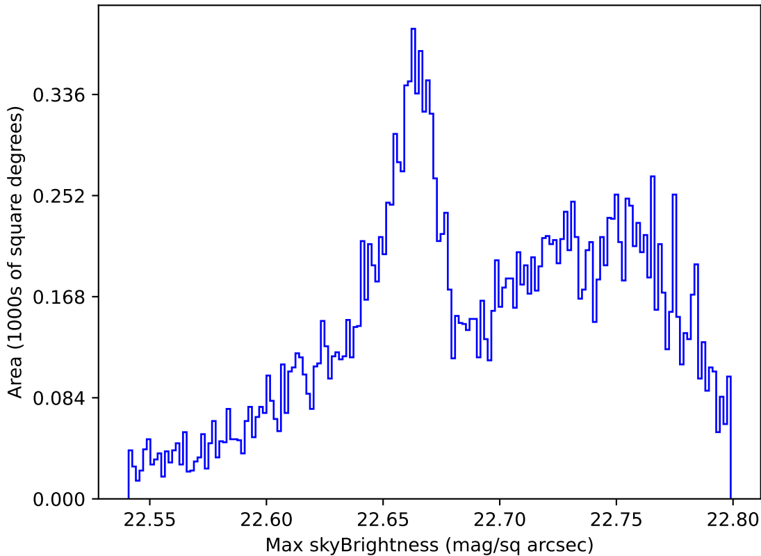
ddf_acor_sf10_lsf20_lsr10_v3.4_10yrs All sky u band: Max skyBrightness
