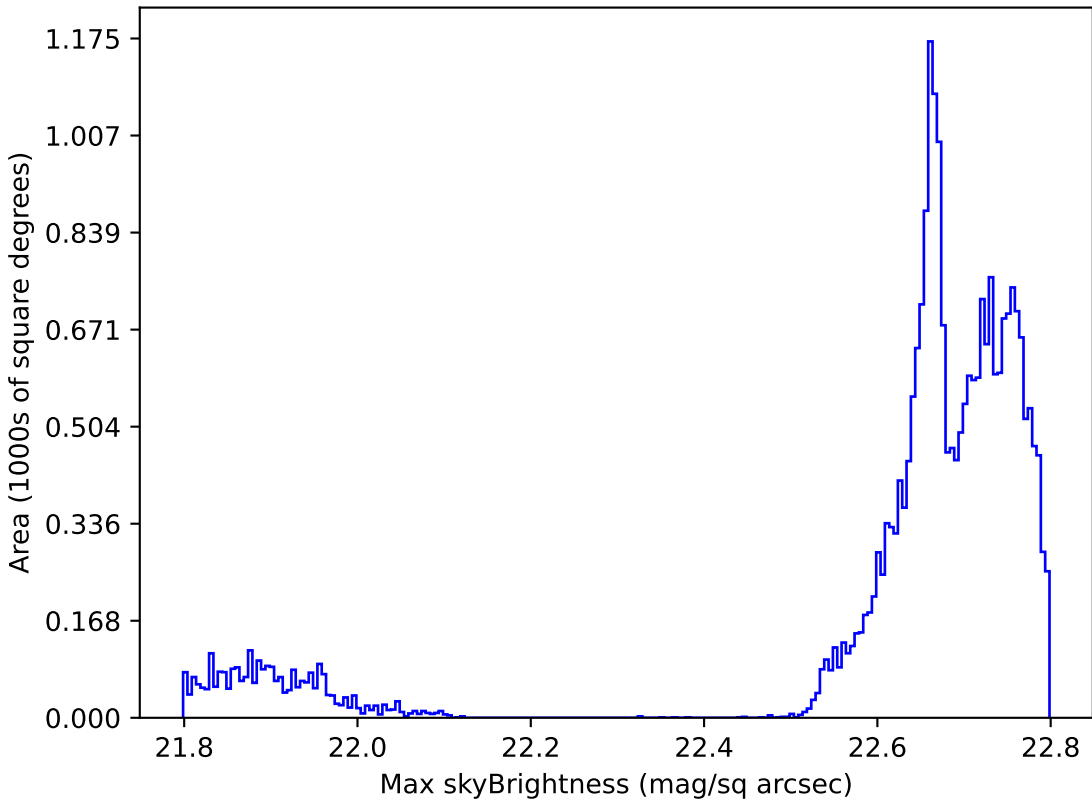
ddf_acor_sf10_lsf20_lsr10_v3.4_10yrs All sky all bands: Max skyBrightness
