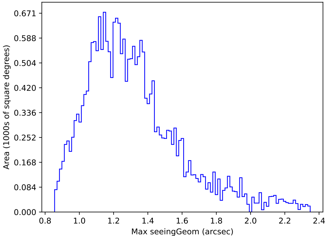
ddf_acor_sf10_lsf20_lsr10_v3.4_10yrs Yr 1 y band: Max seeingGeom
