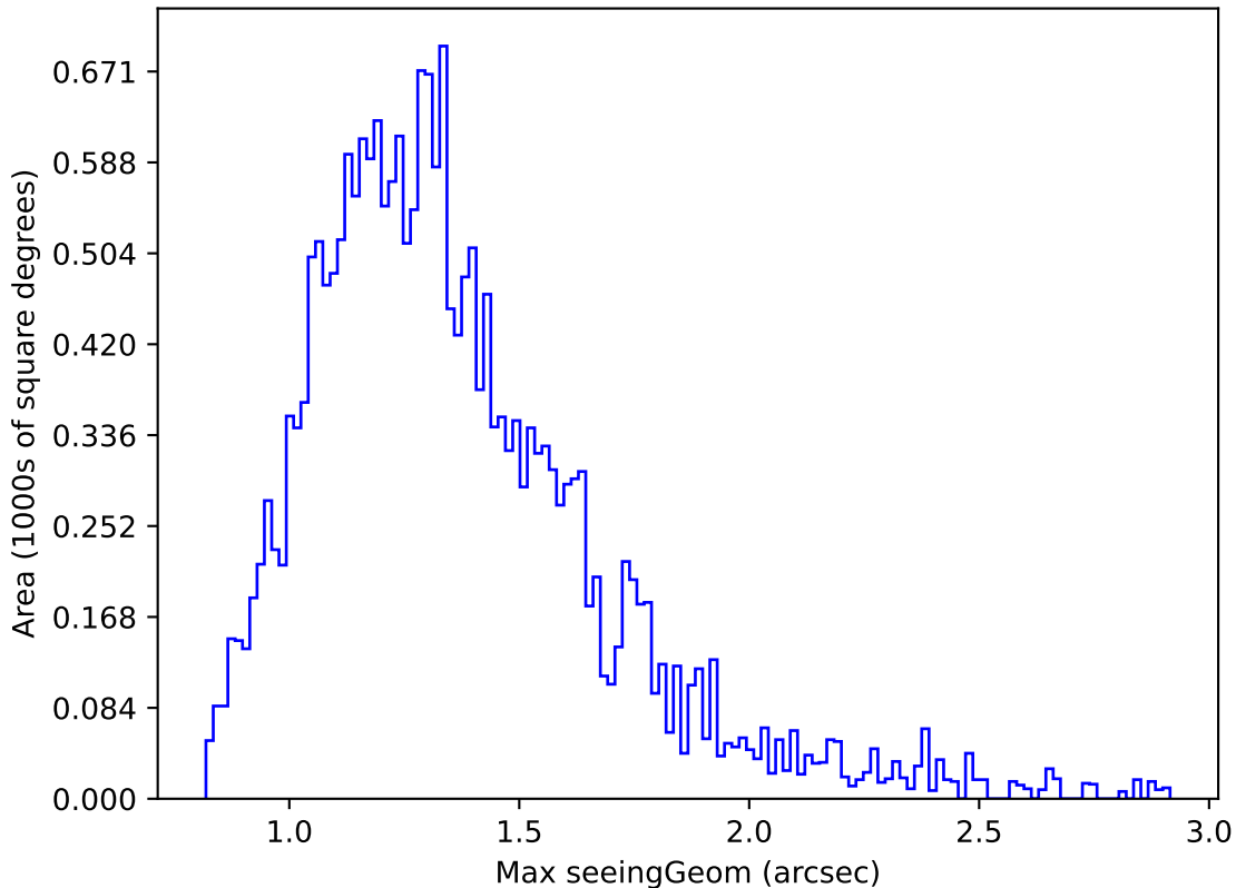
ddf_acor_sf10_lsf20_lsr10_v3.4_10yrs Yr 1 u band: Max seeingGeom
