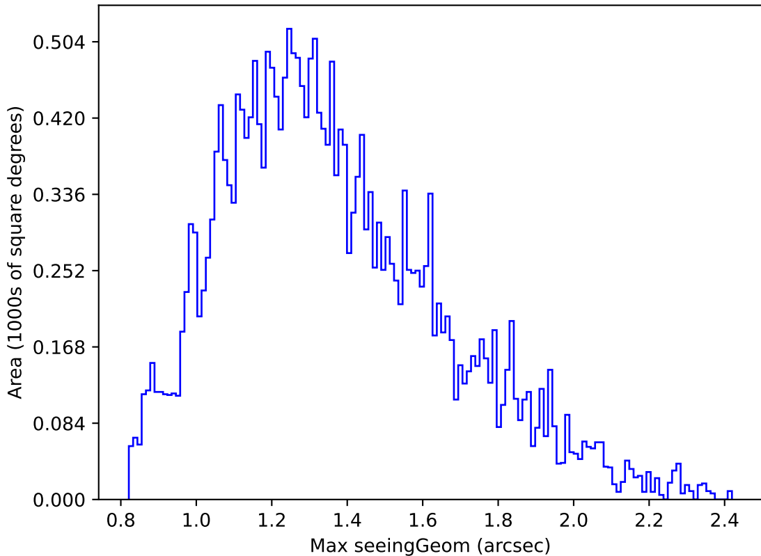
ddf_acor_sf10_lsf20_lsr10_v3.4_10yrs Yr 1 r band: Max seeingGeom
