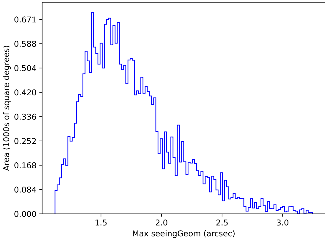
ddf_acor_sf10_lsf20_lsr10_v3.4_10yrs Yr 1 all bands: Max seeingGeom
