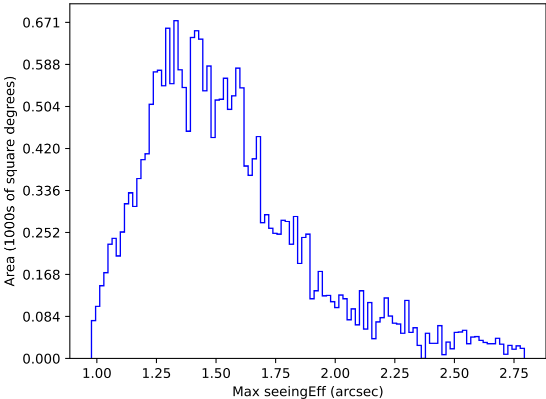
ddf_acor_sf10_lsf20_lsr10_v3.4_10yrs Yr 1 y band: Max seeingEff
