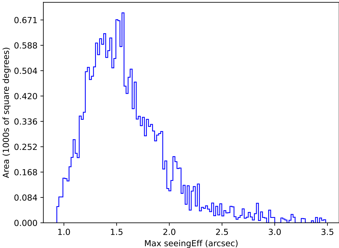
ddf_acor_sf10_lsf20_lsr10_v3.4_10yrs Yr 1 u band: Max seeingEff
