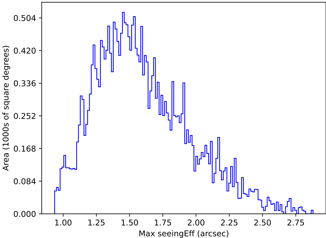
ddf_acor_sf10_lsf20_lsr10_v3.4_10yrs Yr 1 r band: Max seeingEff
