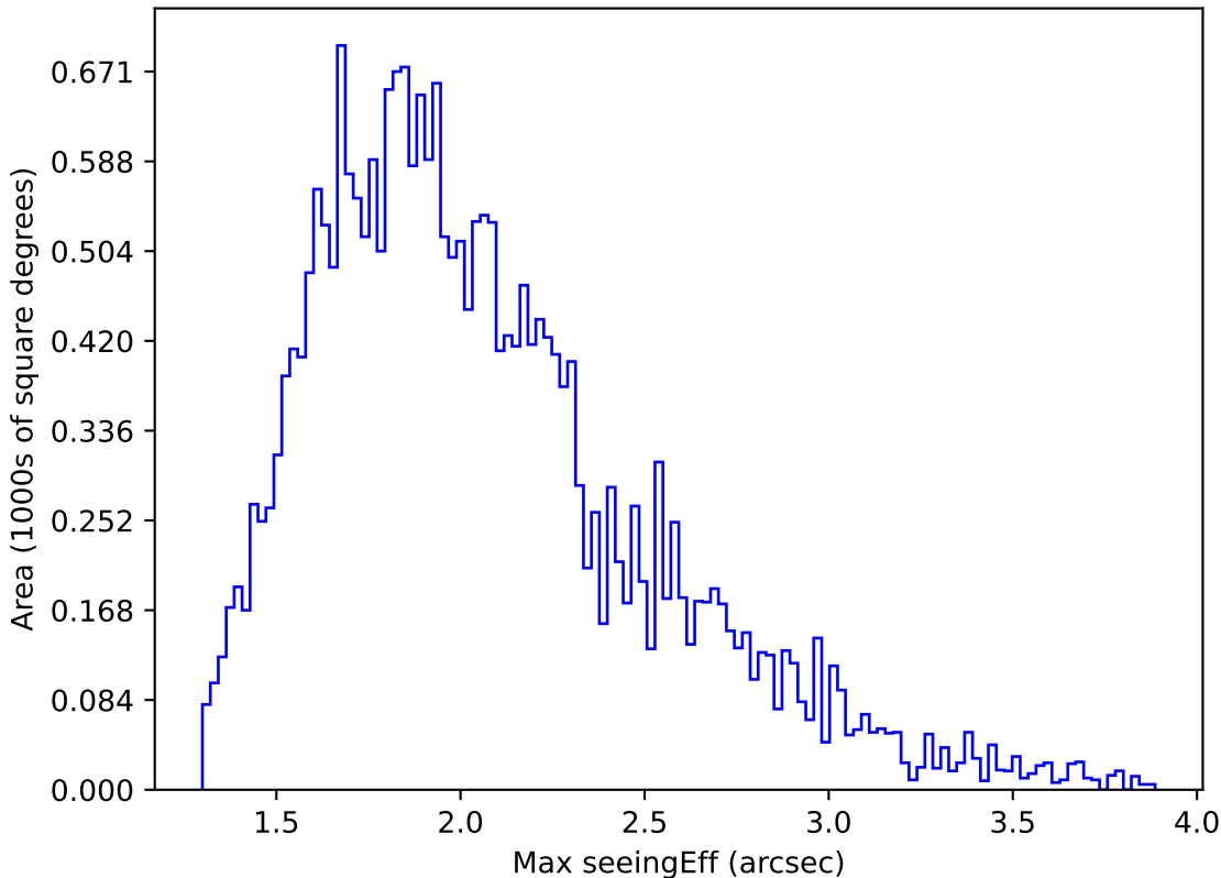
ddf_acor_sf10_lsf20_lsr10_v3.4_10yrs Yr 1 all bands: Max seeingEff
