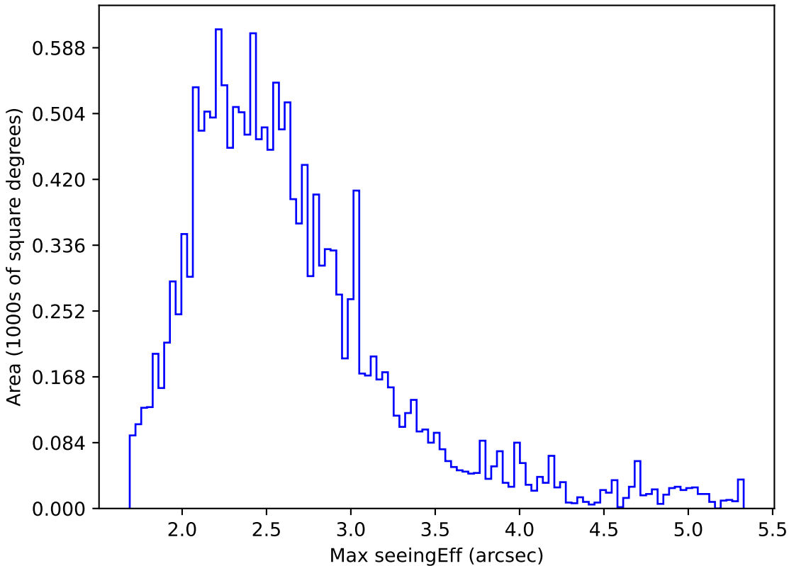
ddf_acor_sf10_lsf20_lsr10_v3.4_10yrs WFD z band: Max seeingEff
