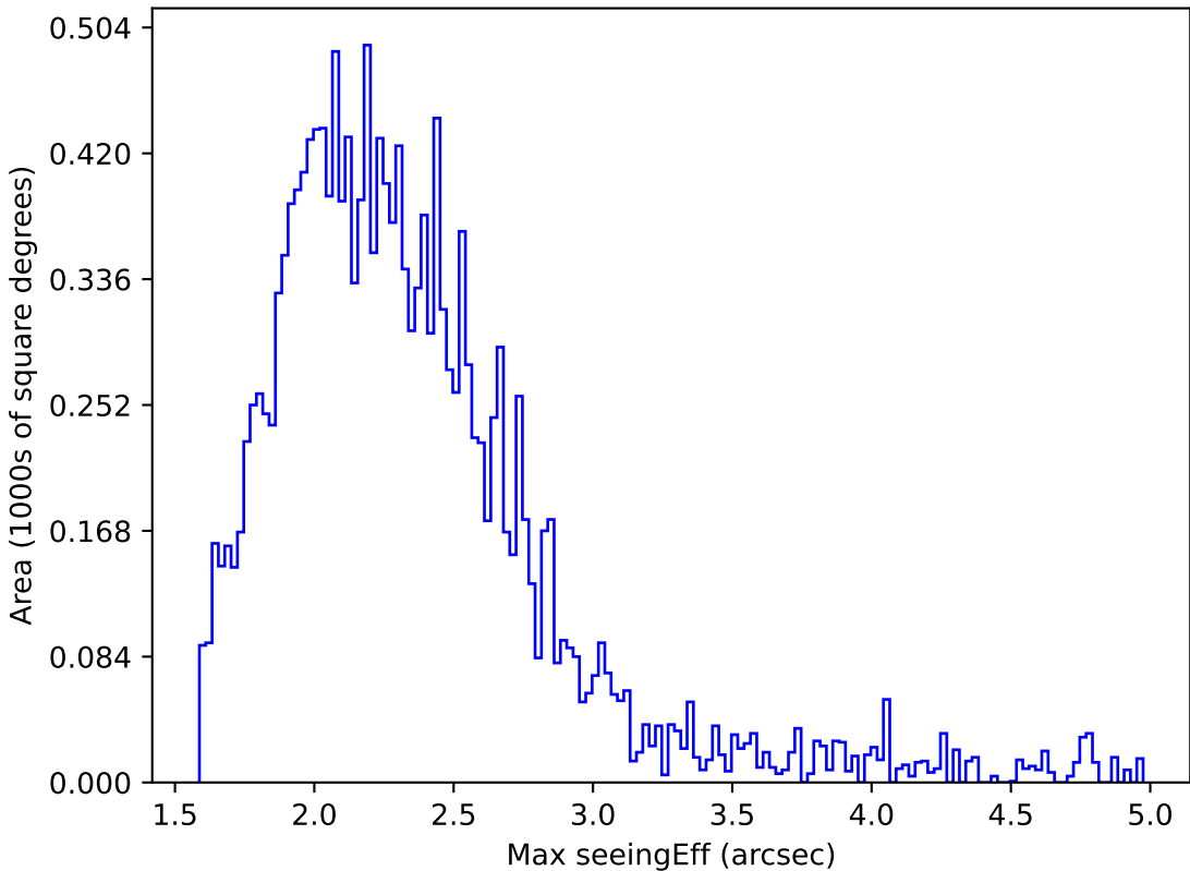
ddf_acor_sf10_lsf20_lsr10_v3.4_10yrs WFD y band: Max seeingEff
