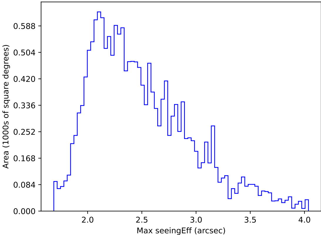
ddf_acor_sf10_lsf20_lsr10_v3.4_10yrs WFD u band: Max seeingEff
