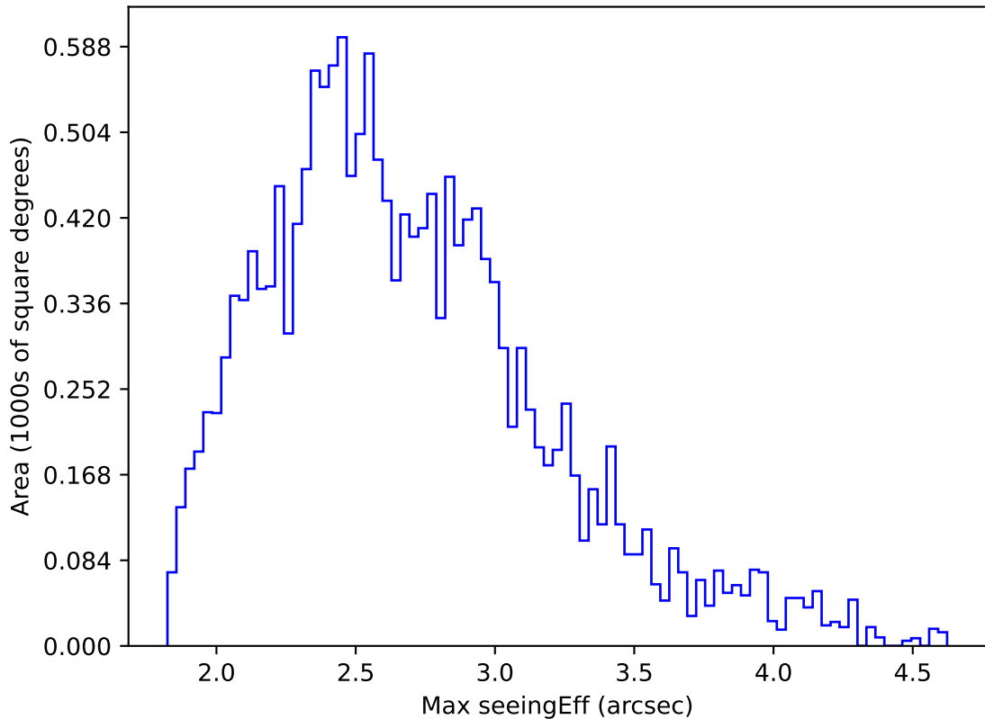
ddf_acor_sf10_lsf20_lsr10_v3.4_10yrs WFD r band: Max seeingEff
