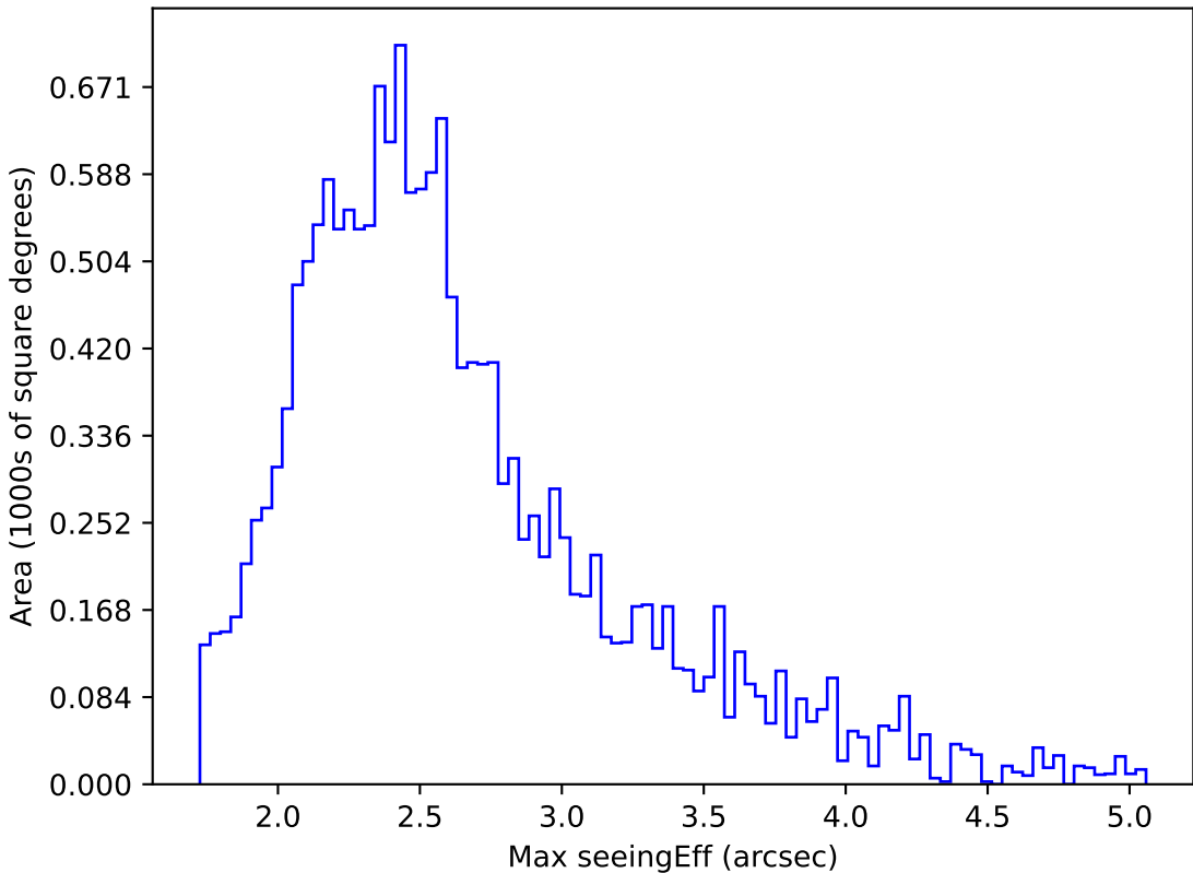
ddf_acor_sf10_lsf20_lsr10_v3.4_10yrs WFD i band: Max seeingEff
