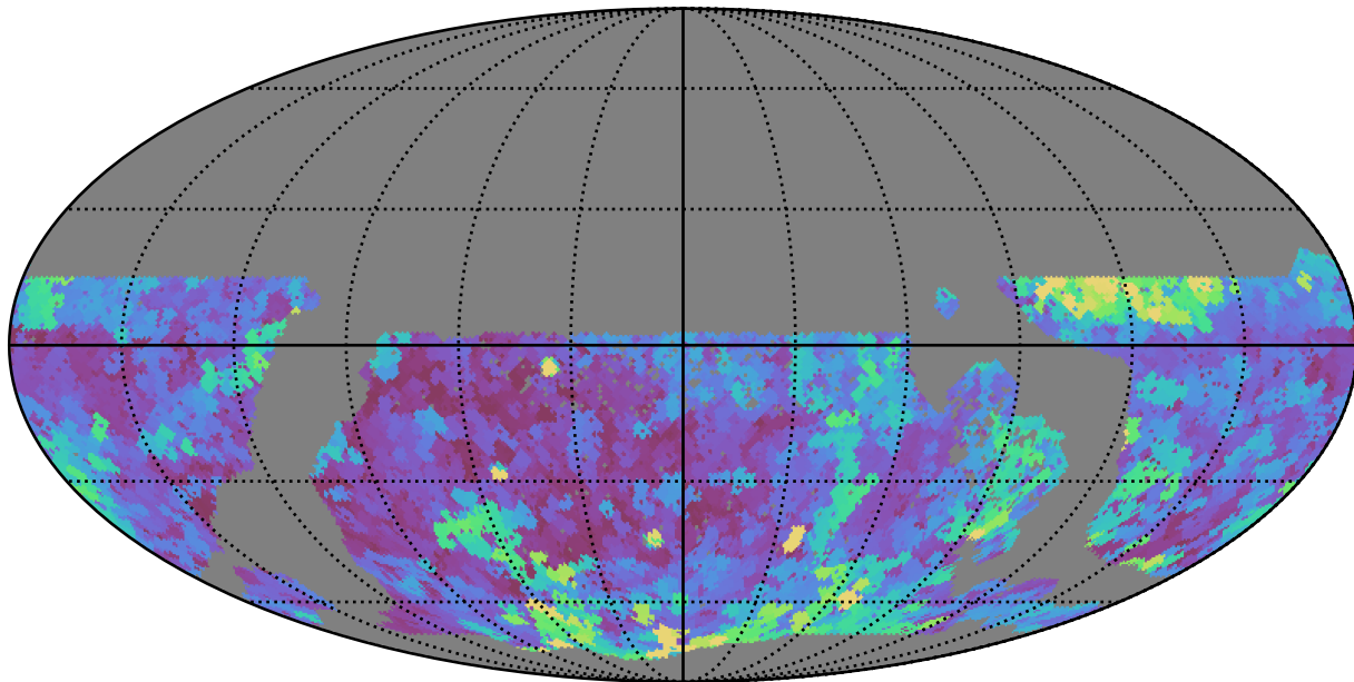
ddf_acor_sf10_lsf20_lsr10_v3.4_10yrs WFD g band: Max seeingEff
