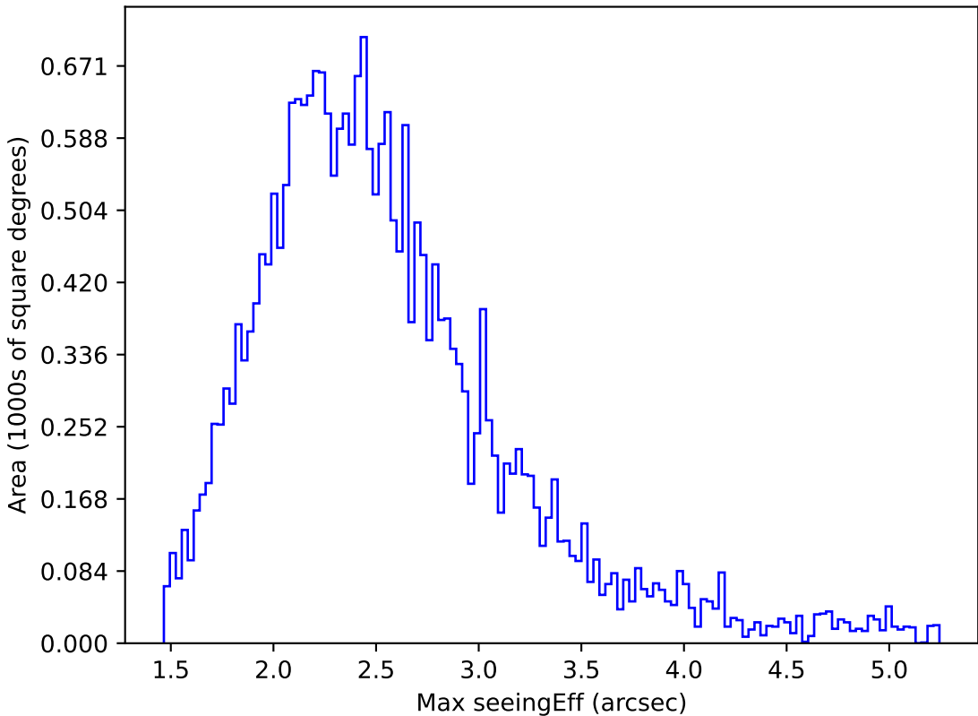
ddf_acor_sf10_lsf20_lsr10_v3.4_10yrs All sky z band: Max seeingEff
