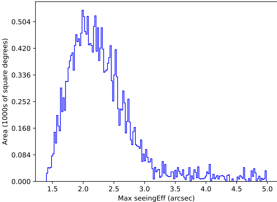
ddf_acor_sf10_ls20_lsr10_v3.4_10yrs All sky y band: Max seeingEff
