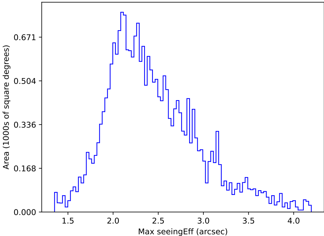
ddf_acor_sf10_ls20_lsr10_v3.4_10yrs All sky u band: Max seeingEff
