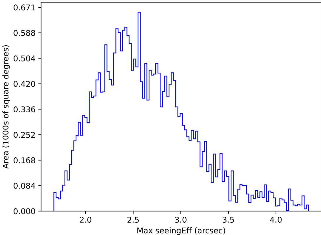
ddf_acor_sf10_lsf20_lsr10_v3.4_10yrs All sky r band: Max seeingEff
