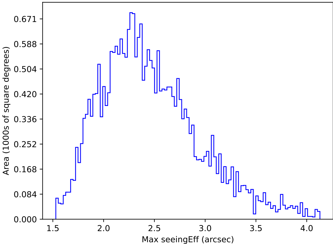
ddf_acor_sf10_ls20_lsr10_v3.4_10yrs All sky g band: Max seeingEff
