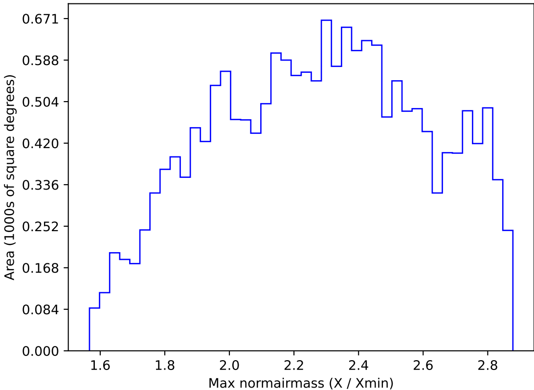
ddf_acor_sf10_lsf20_lsr10_v3.4_10yrs WFD i band: Max normairmass
