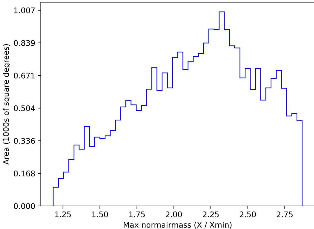
ddf_acor_sf10_ls120_lsr10_v3.4_10yrs All sky z band: Max normairmass
