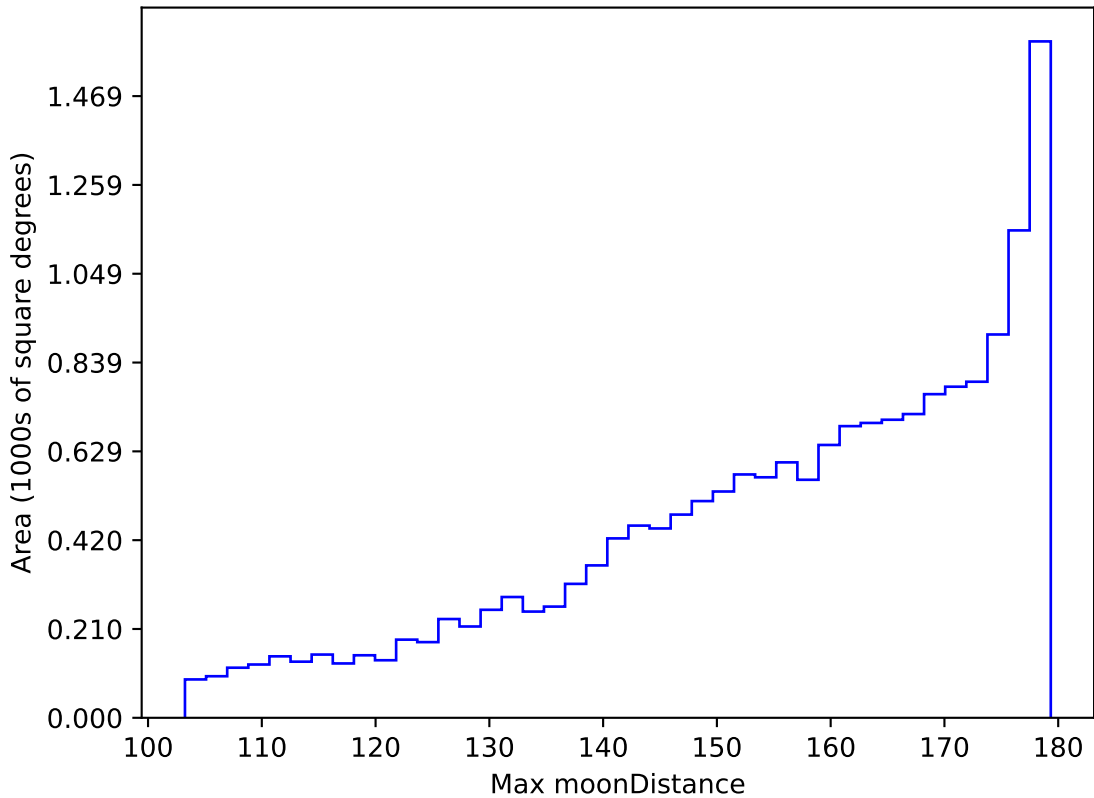
ddf_acor_sf10_lsf20_lsr10_v3.4_10yrs WFD r band: Max moonDistance
