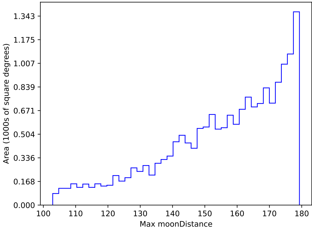
ddf_acor_sf10_lsf20_lsr10_v3.4_10yrs WFD i band: Max moonDistance
