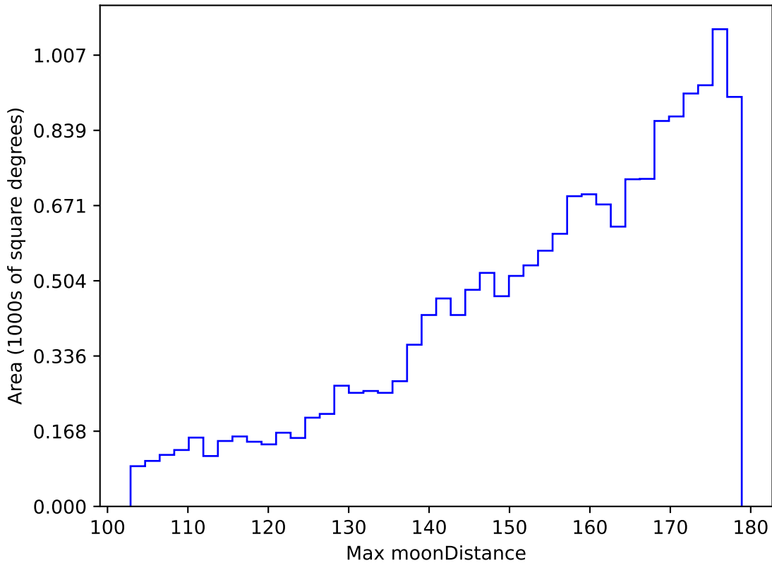
ddf_acor_sf10_lsf20_lsr10_v3.4_10yrs WFD g band: Max moonDistance
